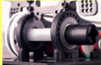
ADJUSTABLE DIFFS WITH COMPOSITE OUTDRIVES
