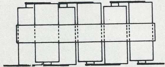
Figure 2a: 6-Cell Hump Pack
