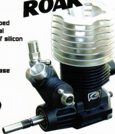
80051 Wasp .12 ROAR Engine (rear exhaust, SG shaft, slide carb.)
