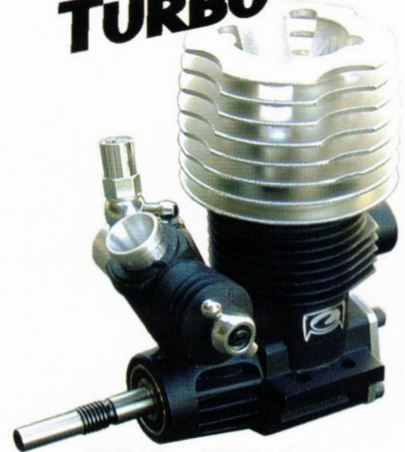
80052 Wasp .12 Turbo Engine (rear exhaust, SG shaft, slide carb.)
